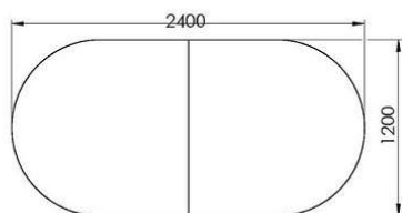
Xenia dining table extendable 240x120(290x120), oval, profile edge HB108015E
